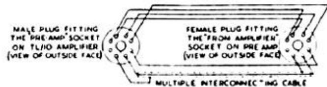
MULTIPLE INTERCONNECTING CABLE
